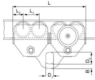
Model HTG, 20.000 kg
