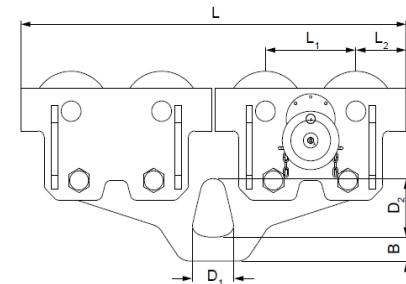
Model HTG, 50.000 kg
