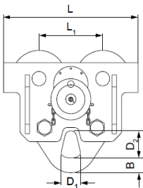
Model HTG, 30.000 kg
