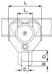
Model HTG, 10.000 kg
