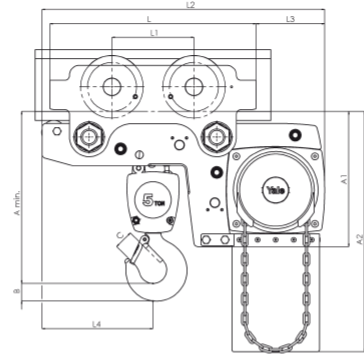
Model Yalelift LHP/LHG, 5.000 kg, çiftli
