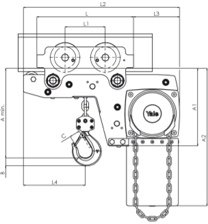
Model Yalelift LHP, 500 - 3.000 kg, tekli
